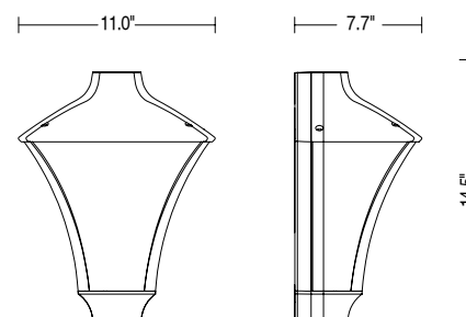
Fixture Dimensions
