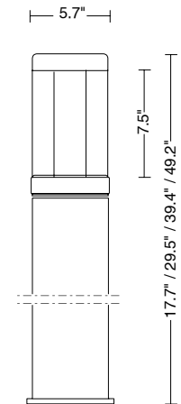
Fixture Dimensions
