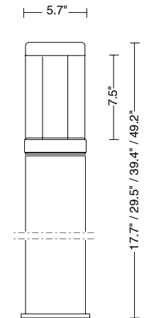
Fixture Dimensions
