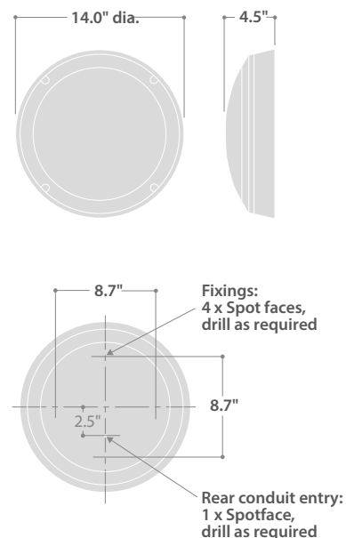
Fixture Dimensions
