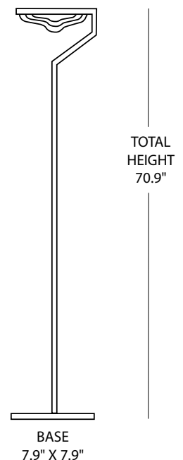
Fixture Dimensions
