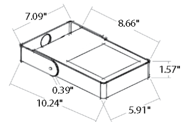
Fixture Dimensions
