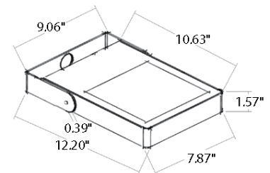
Fixture Dimensions
