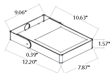
Fixture Dimensions
