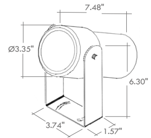
Fixture Dimensions
