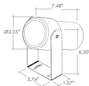
Fixture Dimensions
