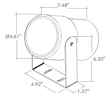
Fixture Dimensions
