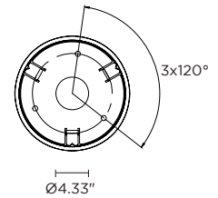
Fixture Dimensions
