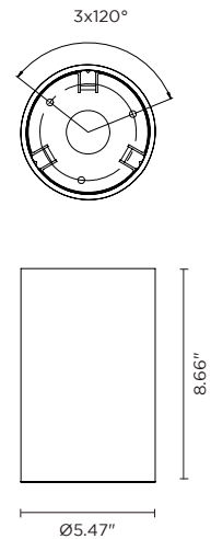
Fixture Dimensions
