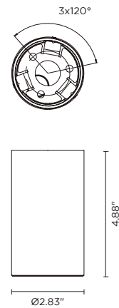
Fixture Dimensions
