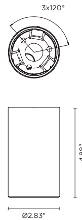
Fixture Dimensions
