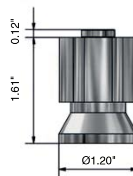
Fixture Dimensions:
