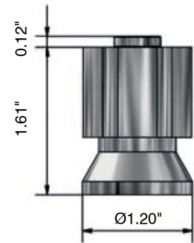
Fixture Dimensions:
