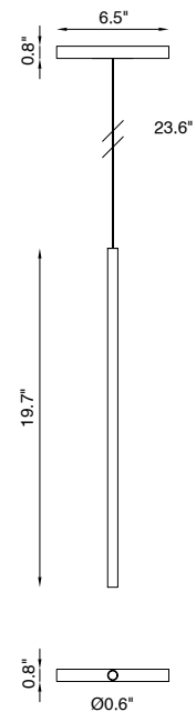
Fixture Dimensions
