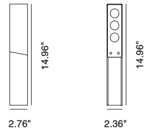
Fixture Dimensions
