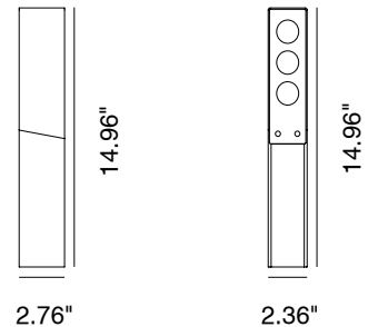
Fixture Dimensions
