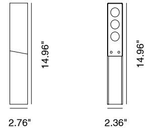
Fixture Dimensions
