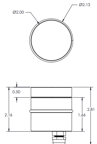
Fixture Dimensions
