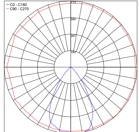
PHOTOMETRIC FILENAME : FLEX M-02 30K 65° - PT5052036N
