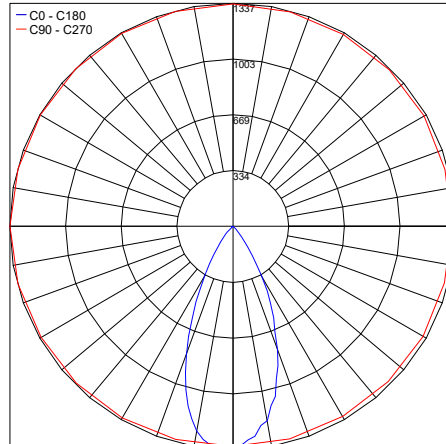
PHOTOMETRIC FILENAME : FLEX M-02 30K 45° - PT5052034N
