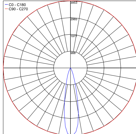
PHOTOMETRIC FILENAME : FLEX M-02 30K 21° - PT5052032N
