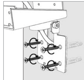
Drill the wall in the traced marks, insert the fixing plugs and align the bracket and screws
