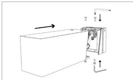
Reassemble device body
