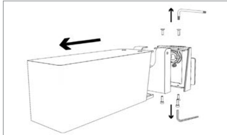
Disassemble device body using T9 Torx key for upper screws and 2.5 mm (0.10") Allen key for lower screws
