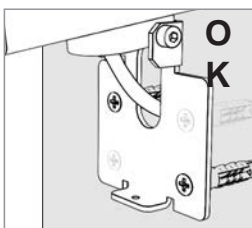
Lock the bracket with at least two alternate screws, guiding the cable through the slots provided
