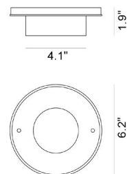
PT50001 Outer Casing For GAME fixture
