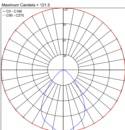
PHOTOMETRIC FILENAME : GINKO 3.3 X 32°X73° [4000K 11W].IES
