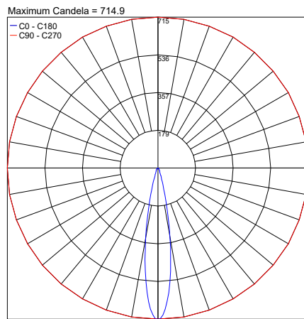
PHOTOMETRIC FILENAME : GINKO 3.3 S 19° [4000K 11W].IES
