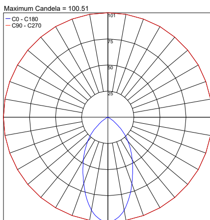
PHOTOMETRIC FILENAME : GINKO 3.3 L 56° [4000K 11W].IES
