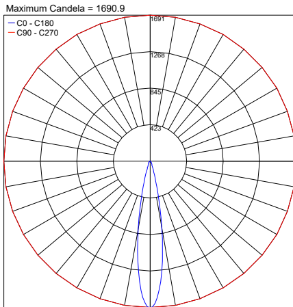
PHOTOMETRIC FILENAME : GINKO 3.3 S 19° [RGBW 11W].IES
