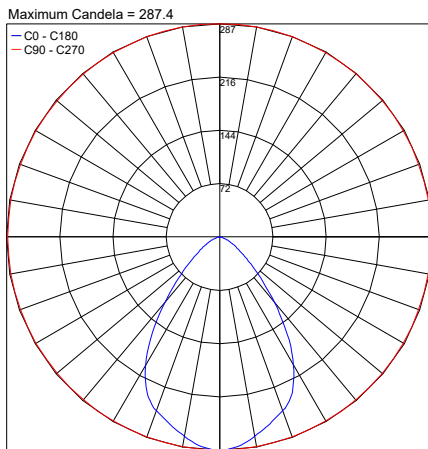
PHOTOMETRIC FILENAME : GINKO 3.3 X 32°X73° [RGBW 11W].IES
