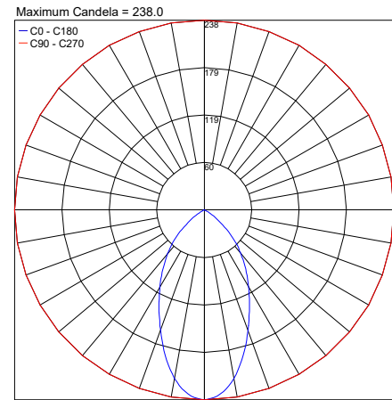
PHOTOMETRIC FILENAME : GINKO 3.3 L 56° [RGBW 11W].IES
