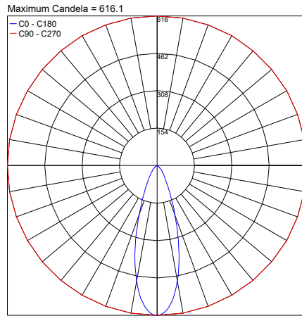
PHOTOMETRIC FILENAME : GINKO 3.3 M 33° [RGBW 11W].IES
