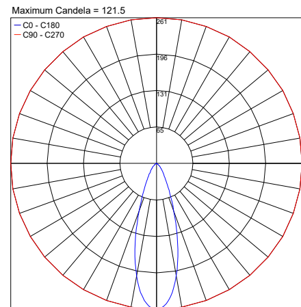
PHOTOMETRIC FILENAME : GINKO 3.3 M 33° [4000K 11W].IES
