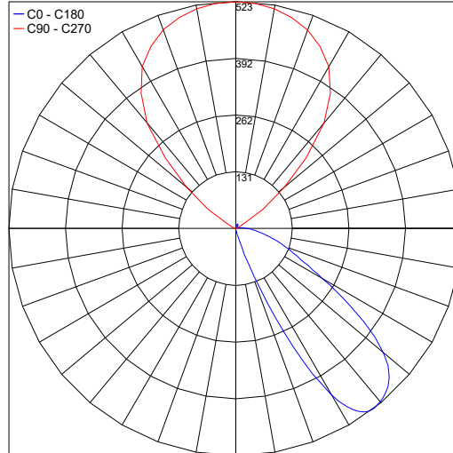
PHOTOMETRIC FILENAME : KANDOVAN H270 SYM 30K - PT2023036B.IES
