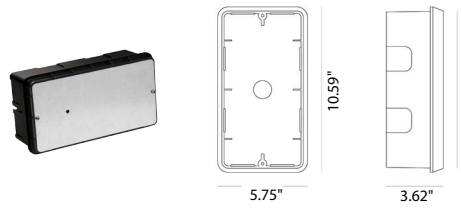
PT50000 Outer Casing for KANDOVAN H270
