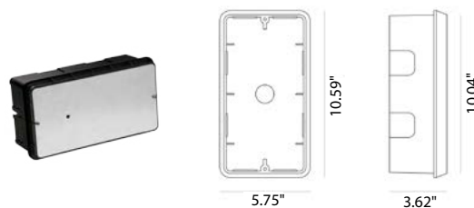
PT50000 Outer Casing for KANDOVAN H270
