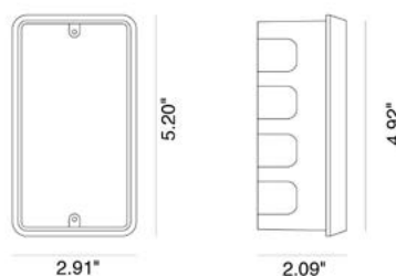
PT50010 Outer Casing for KANDOVAN H130
