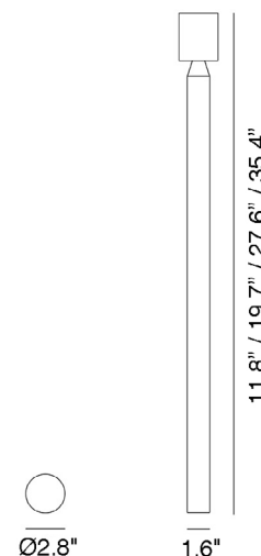
Fixture Dimensions
