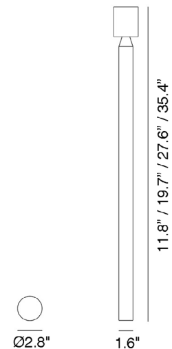
Fixture Dimensions
