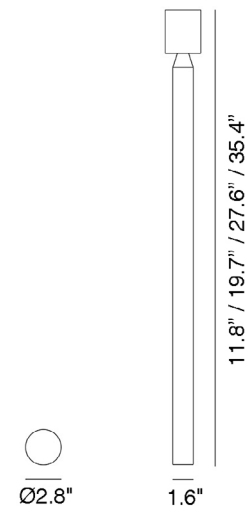
Fixture Dimensions
