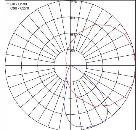
PHOTOMETRIC FILENAME : KRAN M-03 35IN 30K 65°- PT6013369N.IES
