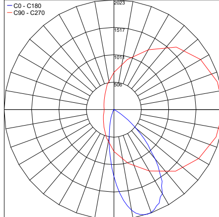
PHOTOMETRIC FILENAME : KRAN M-03 35IN 30K 45°- PT6013349N.IES
