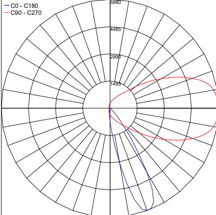
PHOTOMETRIC FILENAME : KRAN M-03 35IN 30K 21°- PT6013329N.IES
