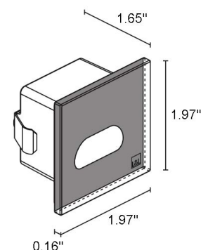
Fixture Dimensions
