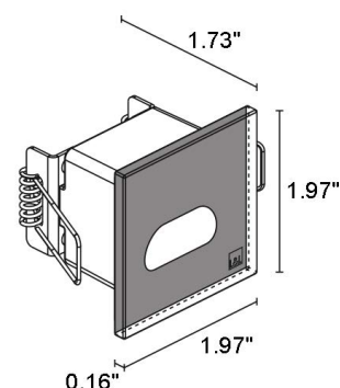
Fixture Dimensions
