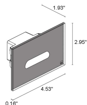
Fixture Dimensions
