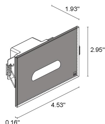
Fixture Dimensions
