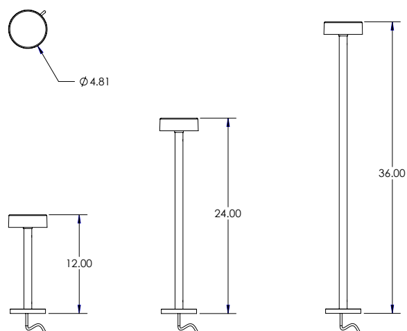
Fixture Dimensions - Spike version on page 2
