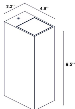
Fixture Dimensions
