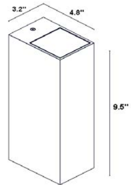
Fixture Dimensions
