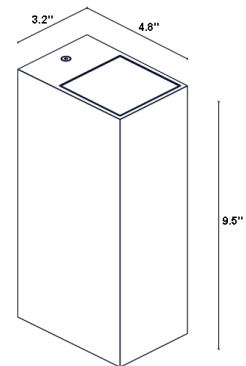
Fixture Dimensions
