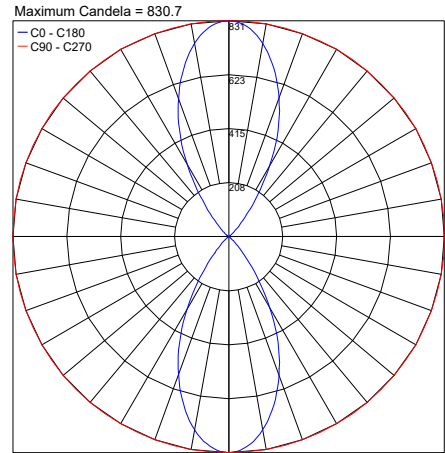
PHOTOMETRIC FILENAME : METOPE_3.2_DD_3000K_19W.IES
