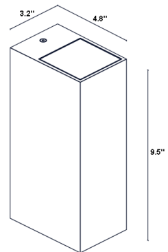
Fixture Dimensions
