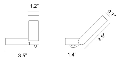
Fixture Dimensions
