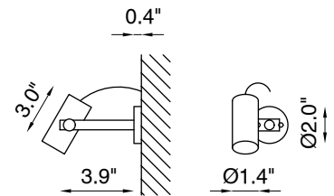
Fixture Dimensions
