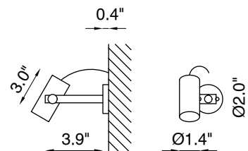
Fixture Dimensions
