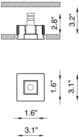
Fixture Dimensions
