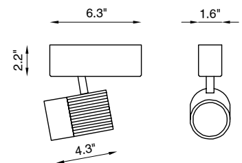
Fixture Dimensions
