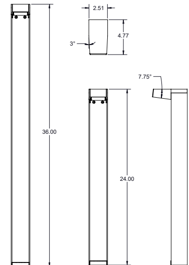
Fixture Dimensions
