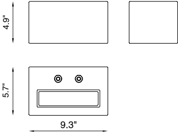
Fixture Dimensions
